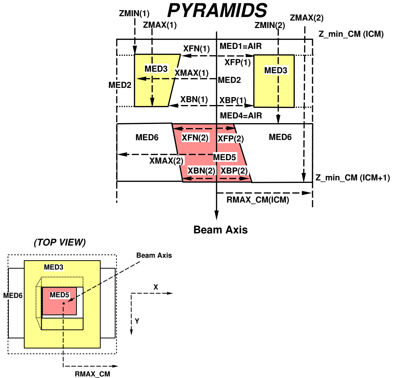
Figure 31: A PYRAMIDS component module with 2 layers (ISCM_MAX=2). Within a layer i , the front of the central region is specified by XFP(i) , XFN(i) , YFP(i) , YFN(i) , and the back is defined by XBP(i) , XBN(i) , YBP(i) , YBN(i) . The central region's inner faces are the planes connecting rectangle defining the front of the region with that defining the back of the region. The X and Y outer edges of layer i are defined by XMAX(i) and YMAX(i) respectively. The figure does not show the Y dimensions ( i.e. YFN(i) , YFP(i) , YMAX(i) , etc. ), however the Y dimensions are evident in the top view. Layers must be separated by at least 0.01cm ( ZMIN(i+1)-ZMAX(i) \geq 0.01cm ). By setting IFILL=1 , the user can set the medium filling the central and outer regions in each layer (MED2 and MED5). The gaps between layers are assumed to be filled with air.
