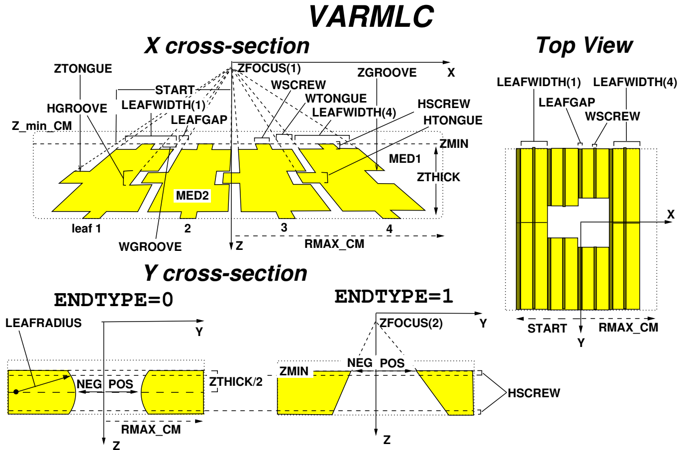
Figure 35: A VARMLC component module with 4 leaves (NUM_LEAF=4) opening in the Y direction (ORIENT=0). The X cross-section (perpendicular to the leaf direction) shows the widths of the leaves (LEAFWIDTH(1)...LEAFWIDTH(4)) and the dimensions of the leaf gap (LEAFGAP), tongue-in-groove mechanism (WGROOVE, HGROOVE, WTONGUE, HTONGUE) and the driving screws (WSCREW, HSCREW) as input by the user. The user also sets the position of the top of the tongue, ZTONGUE, and the top of the groove, ZGROOVE, with the restriction that the tongue and groove cannot overlap. If ZTONGUE=ZGROOVE=0 then the tongue and groove are centred at Z = ZMIN + ZTHICK/2 . For restrictions on leaf gap and tongue-in-groove inputs, see the detailed description of input parameters below. Note that all leaf side surfaces are focused at ZFOCUS(1) and that horizontal dimensions (WGROOVE, WTONGUE, WSCREW, START) are all given at ZMIN. Due to LEAFGAP and varying LEAFWIDTH the leaves may not be symmetric about the Z axis, although START can be set to give approximate symmetry. Also note that the medium in regions beyond the leaves perpendicular to the leaf direction defaults to MED1, the medium of the openings and air gaps. Y cross-sections are shown for leaves with rounded ends (ENDTYPE=0) and straight ends (ENDTYPE=1). For rounded ends, the user inputs the radius of the ends (LEAFRADIUS) and, for each leaf, the minimum and maximum coordinates of the leaf opening at Z = ZMIN + ZTHICK/2 (NEG, POS). The end radius is always assumed to originate at Z = ZMIN + ZTHICK/2 . For straight leaf ends, the user inputs the Z focus of the ends (ZFOCUS(2)) and, for each leaf, the minimum and maximum coordinates of the opening at Z = ZMIN (NEG, POS).
