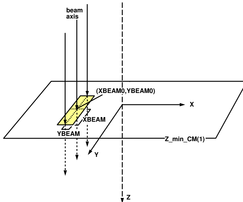
Figure 10: Parallel rectangular beam (ISOIRC=6) showing the beam centre (XBEAM0,YBEAM0) and the X and Y half-widths (XBEAM,YBEAM).
